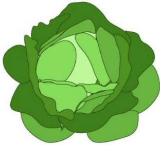
Cabbage
