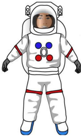
Astronaut
