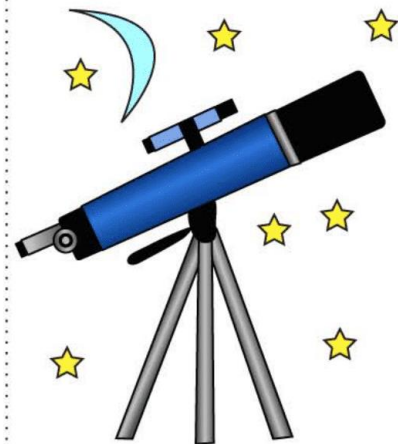
Telescope
