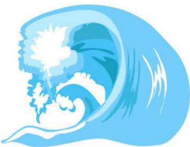
Wave
