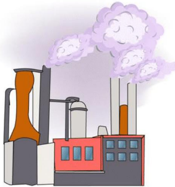
Air pollution
