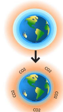
Greenhouse effect
